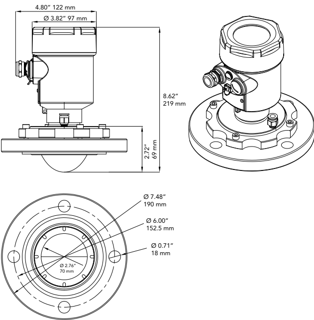
Swivel Flange with Air Purge, 3"
