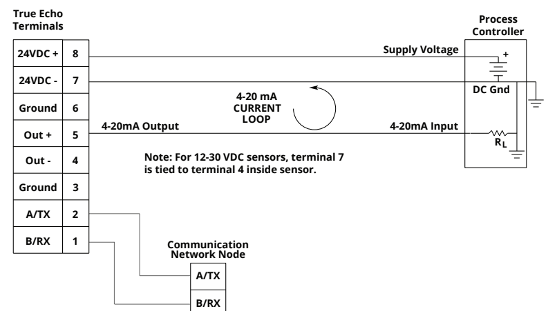
12-30 VDC Power
