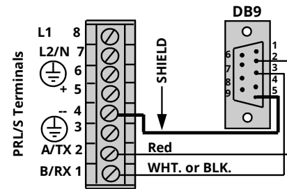
RS-232 SERIAL CONNECTION TO PC
