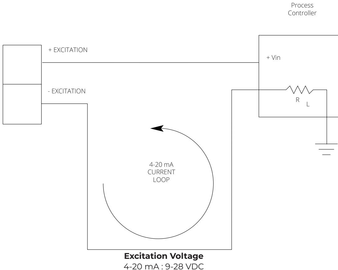
Typical 4-20 mA Circuit
