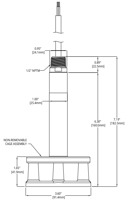
PT-500 with Welded Anti-snag Cage
