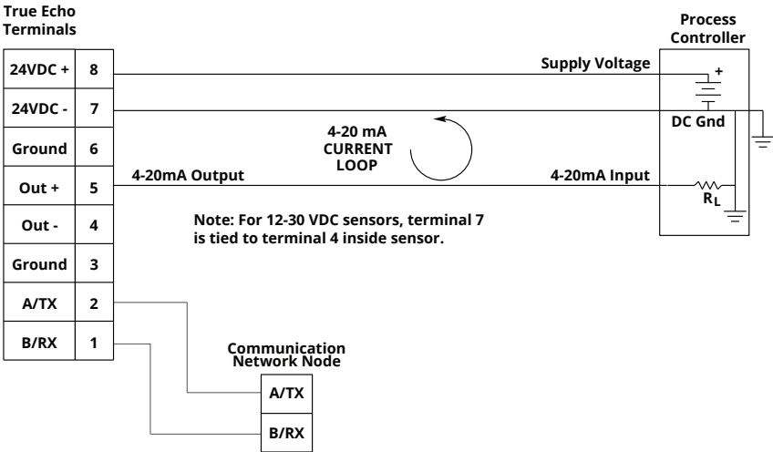
12-30 VDC Power
