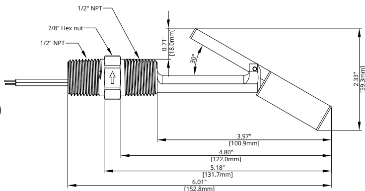
FS-500...P1P1 (open)
