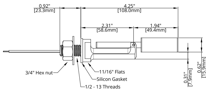
FS-500...P58 (closed)
